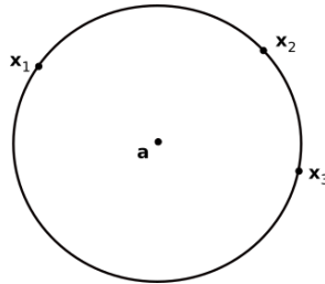
Figure 1. The three distinct, noncollinear points x_1, x_2, x_3 of a given plane are shown as lying on a circle of center point a . The proof of the fact that these points do lie on a circle will be demonstrated by solving for the coordinates of the center point a as functions of the three given points.
